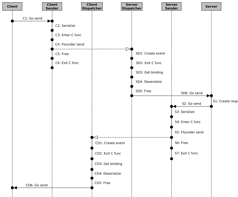
Figure 4.20: Sequence diagram for a single round-trip of a message traversing over the integrated channels. The dashed arrows indicate communication happening over Flounder.
