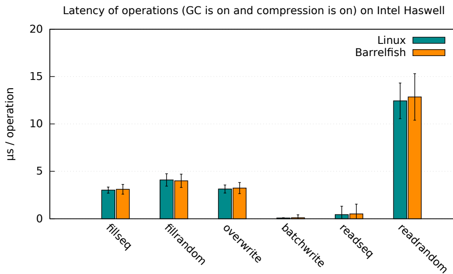
Figure 4.8: Goleveldb benchmark results on Intel Haswell measured in micro seconds when outliers are filtered out.
