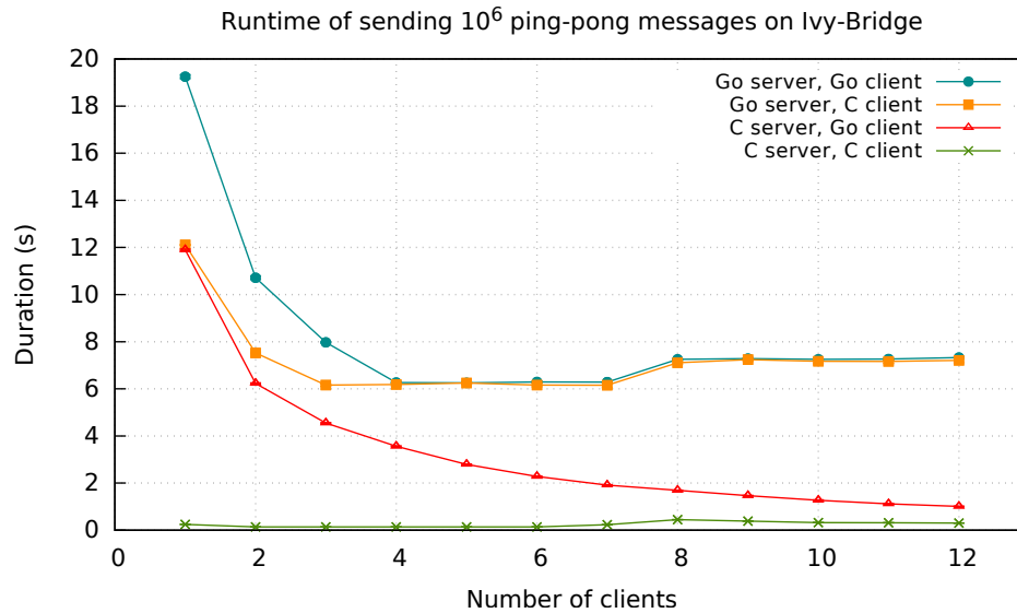
Figure 4.18: Runtime of the ping-pong benchmark when the number of clients increases. Each client sends \frac{10^6}{\text{number\_of\_clients}} requests.
