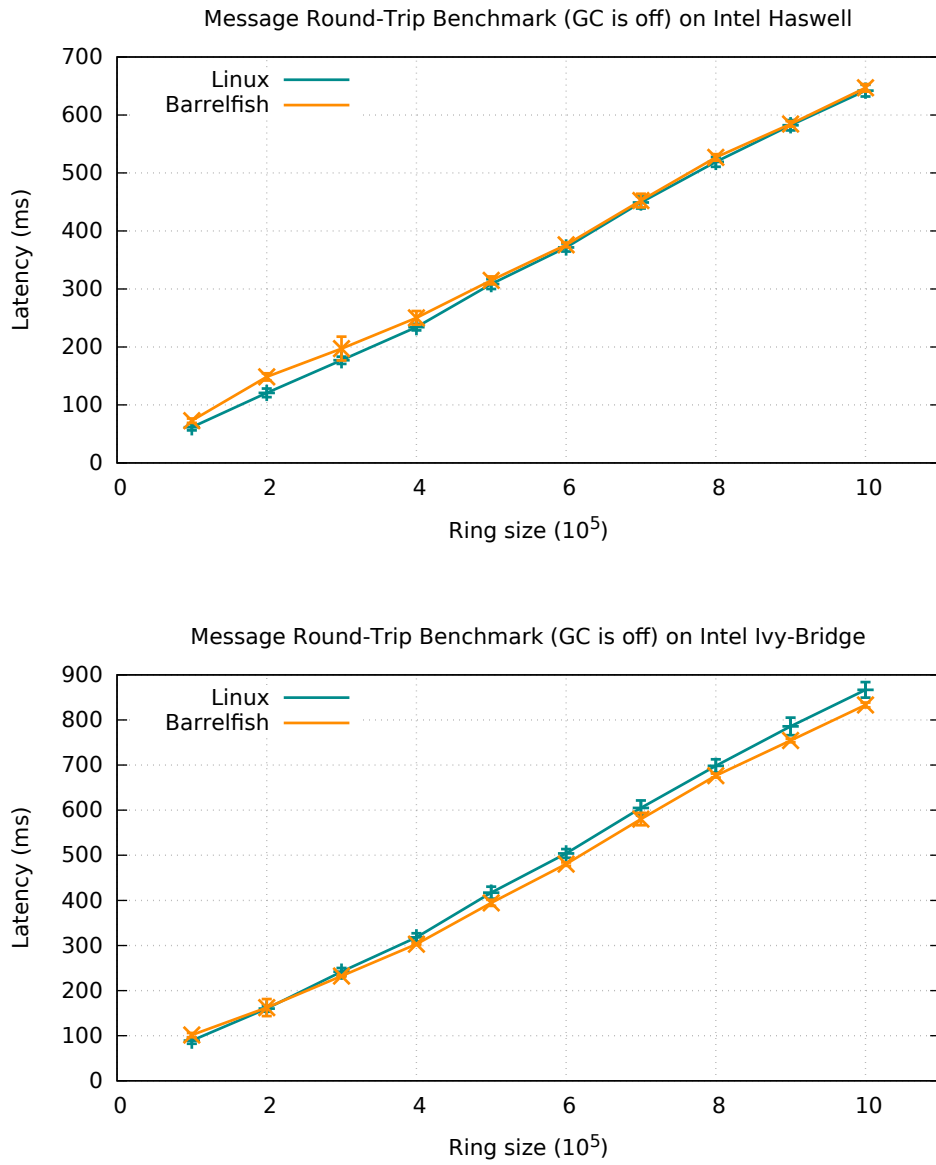
Figure 4.12: The concurrency benchmark results on Intel Ivy-Bridge and Intel Haswell. GC is disabled.
