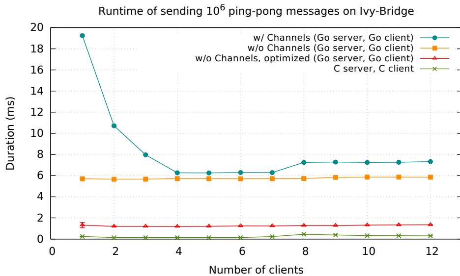
Figure 4.21: Runtime of the ping-pong benchmark when the optimizations are applied.
