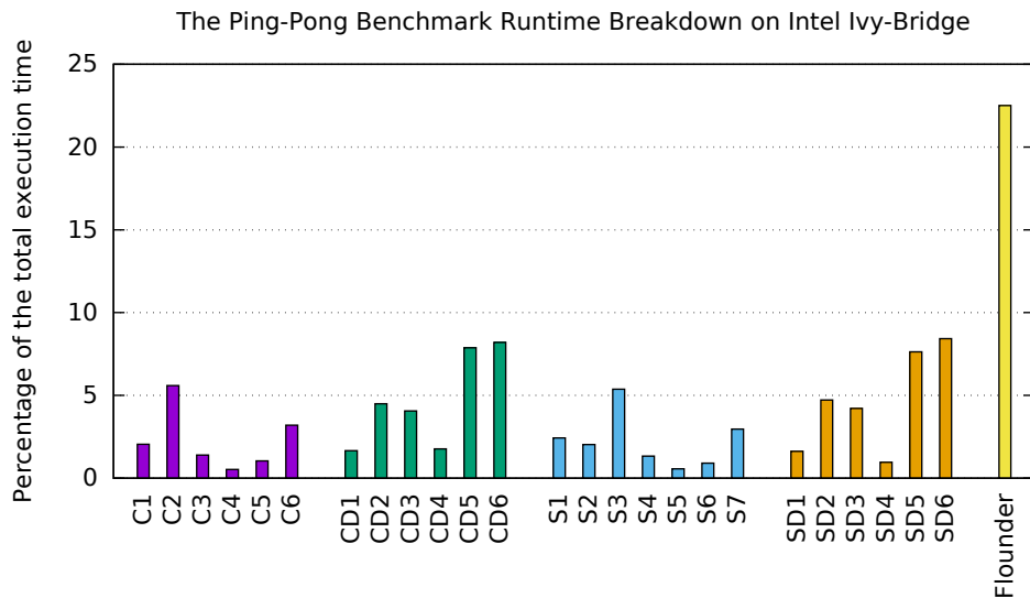
Figure 4.19: Runtime breakdown of the ping-pong benchmark when both server and client are implemented in Go and there is only one client. The breakdown is for a single request-response pair measured over 10^6 samples.
